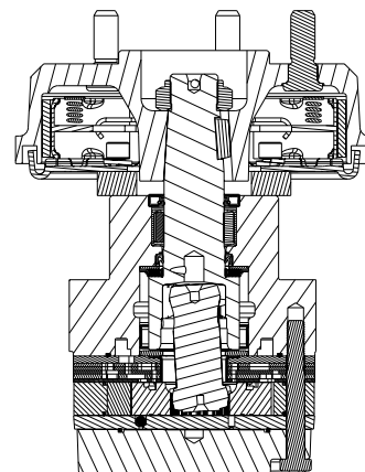
430/431 - Hydraulic Motor With Heavy Duty Bearing
