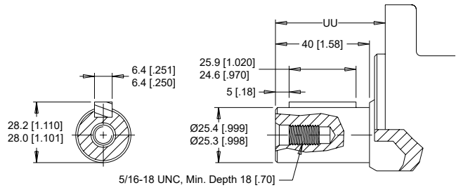
10 1" Straight
