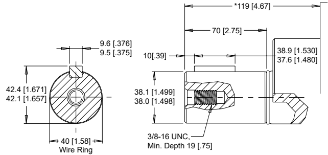
30 1-1/2" Straight
