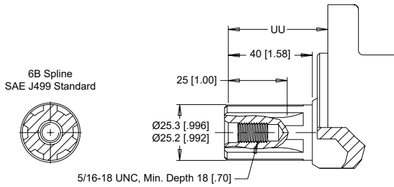
02 1" 6B Spline
