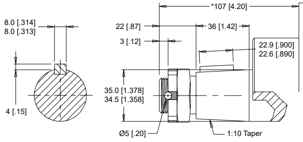
28 35mm Tapered
