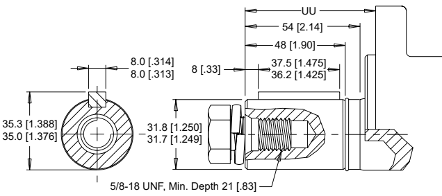
07 1-1/4" Straight Extended
