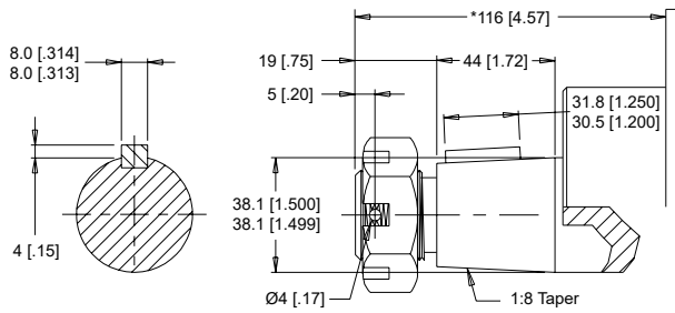
31 1-1/2" Tapered
