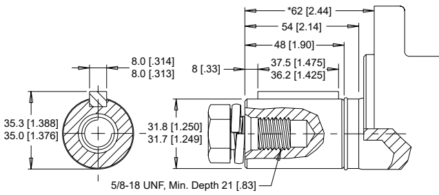
07 1-1/4" Straight
