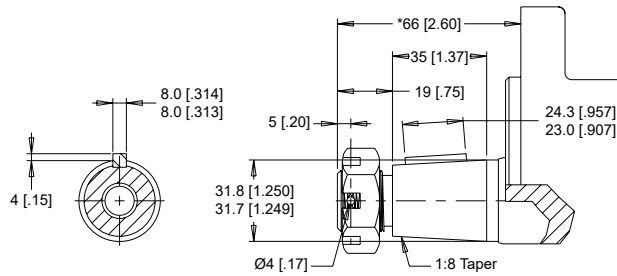
25 1-1/4" Tapered
