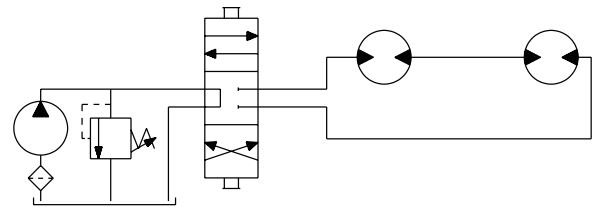
SERIES CIRCUIT
