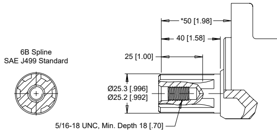
03 1" 6B Spline
