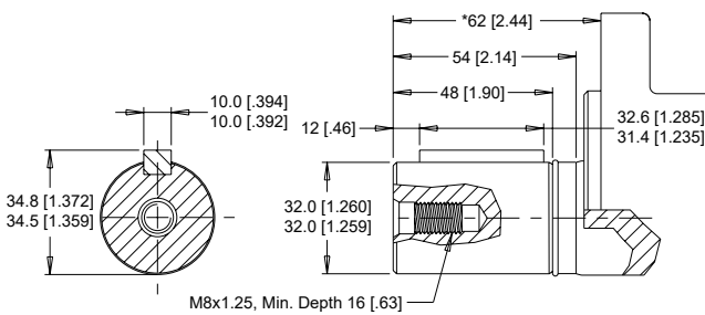
08 32mm Straight
