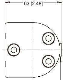
Drain Port: JKB, JLB - G1/8, Min. Depth 8 [.315] JK5, JL5 - 3/8-24UNF, Min. Depth 10 [.394]
