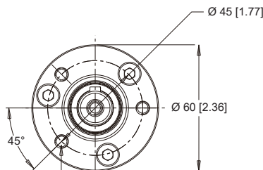
JMB, JM5 - (3) M6 x 1, Min. Depth 10 [.394] JNB, JN5 - (3) 1/4-28 UNF, Min. Depth 10 [.394]
