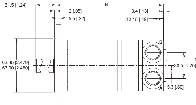
Drain Port: LKB - G1/8, Min. Depth 8 [.315] LL5 - 3/8-24UNF, Min. Depth 10 [.394]
