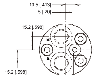
Drain Port: JMB, JNB - G1/8, Min. Depth 8 [.315] JM5, JN5 - 3/8-24UNF, Min. Depth 10 [.394]
