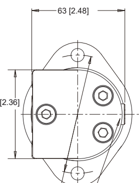
Drain Port: LKB - G1/8, Min. Depth 8 [.315] LL5 - 3/8-24UNF, Min. Depth 10 [.394]
